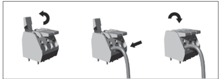
Figure 21 Connection of Terminal Type 3
