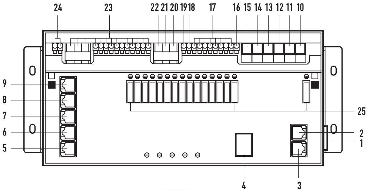
Figure 8 Front panel of PM335J-2 Transformer Unit
