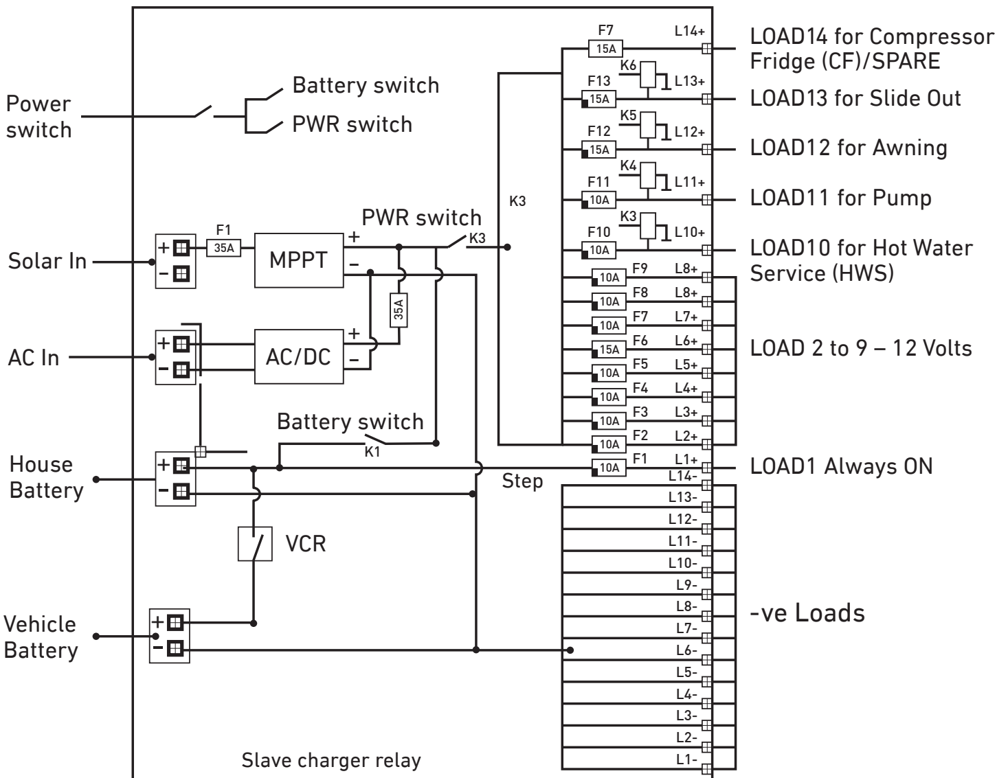
Figure 2 System Schematic
