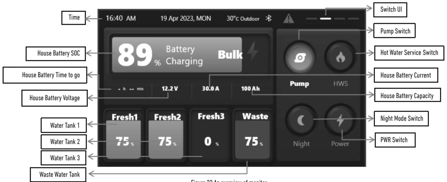
Figure 23 An overview of monitor
