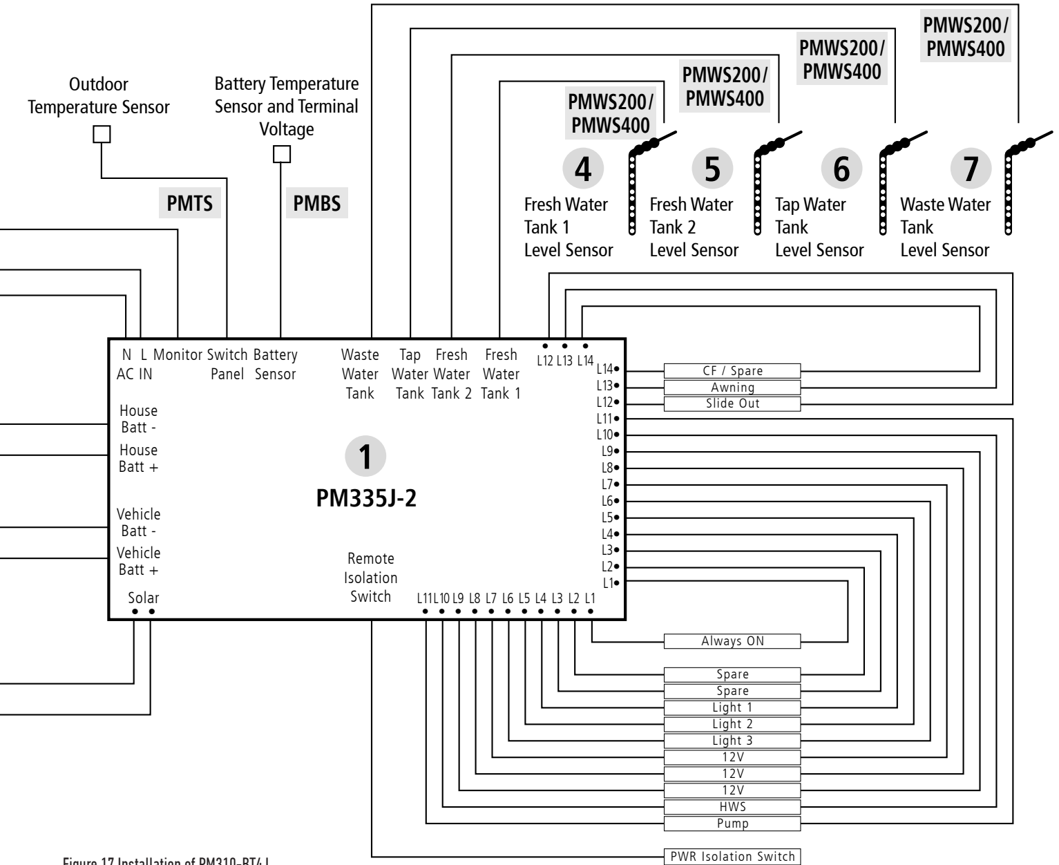
Figure 17 Installation of PM310-BT4J
