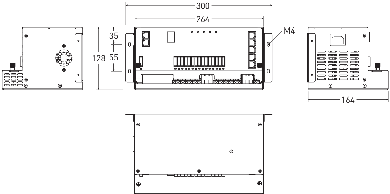
Figure 9 Dimension of PM335J-2 (Unit: mm)
