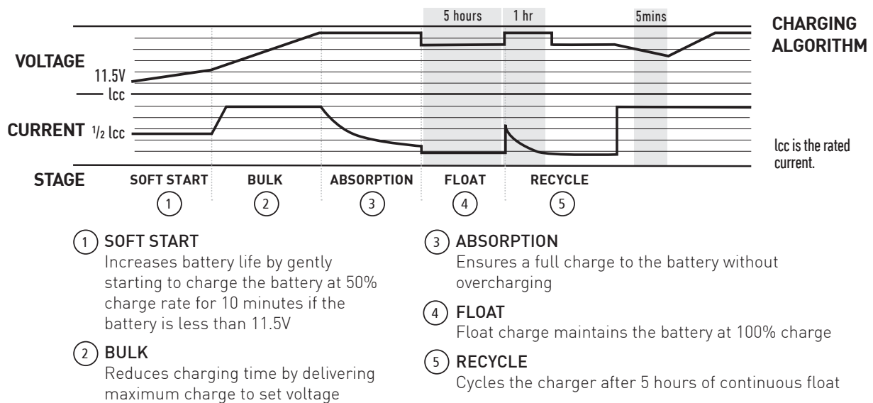
Figure 6 Charging Algorithm
