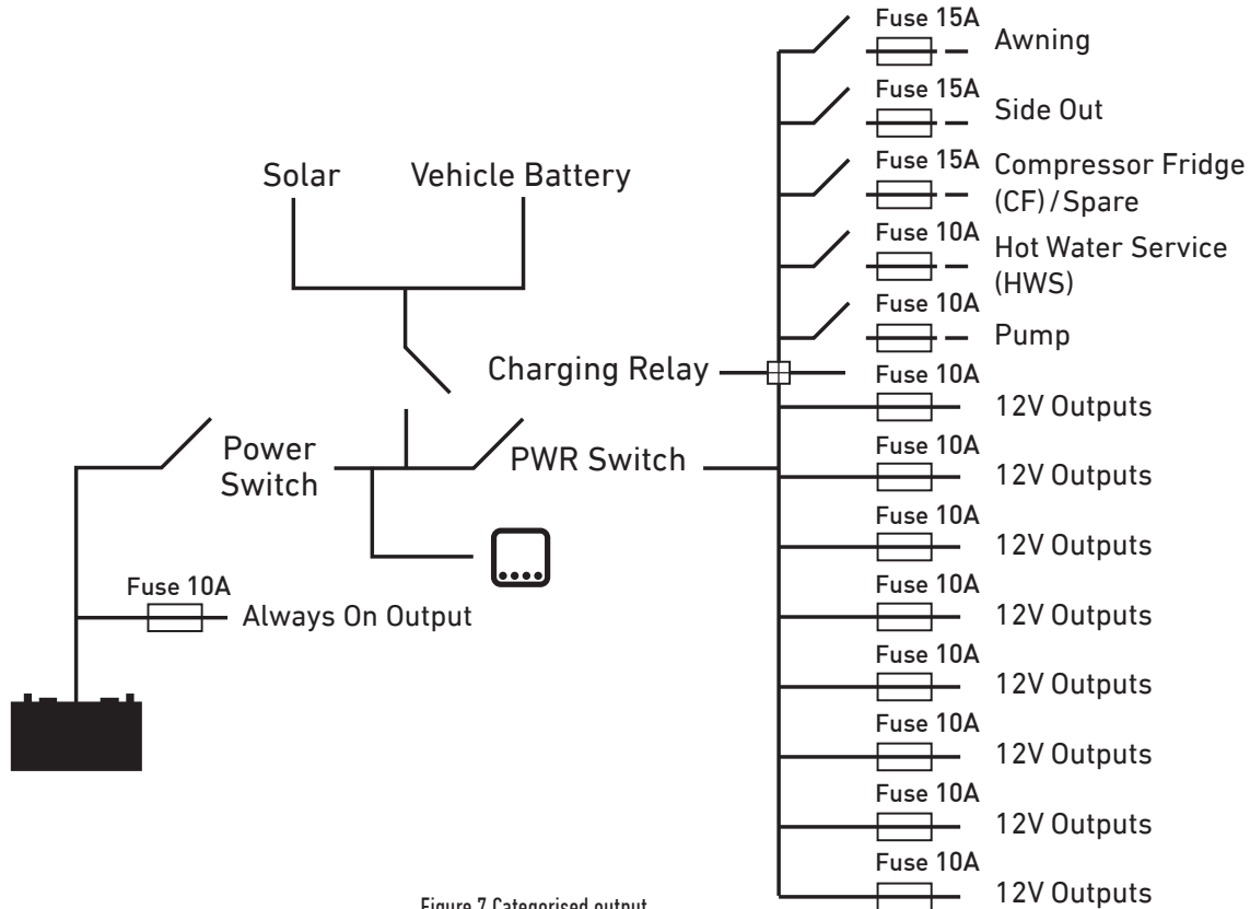
Figure 7 Categoricalised output
